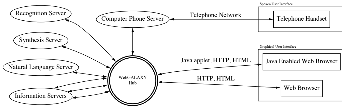
Figure 2: WebGALAXY Architecture
