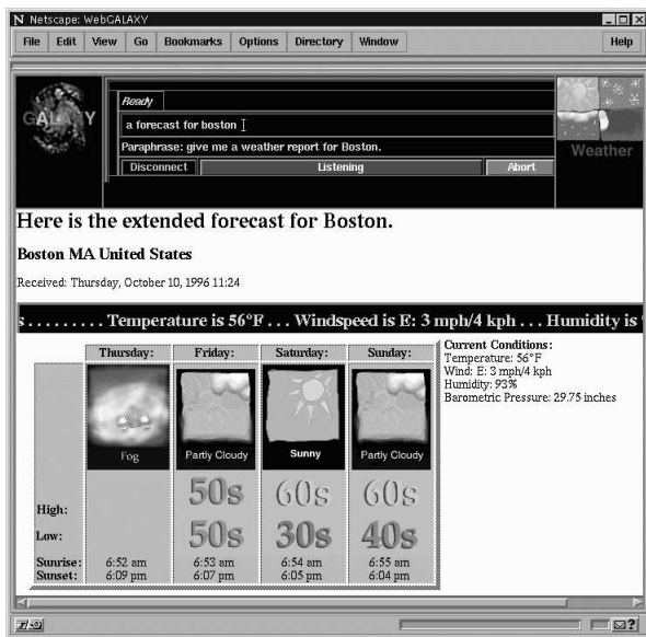
Figure 3: Java-based graphical interface
